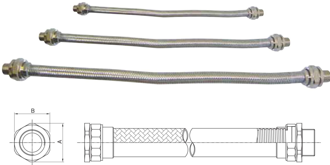
Type of Explosion-Proof Flameproof (Ex d IIC)
